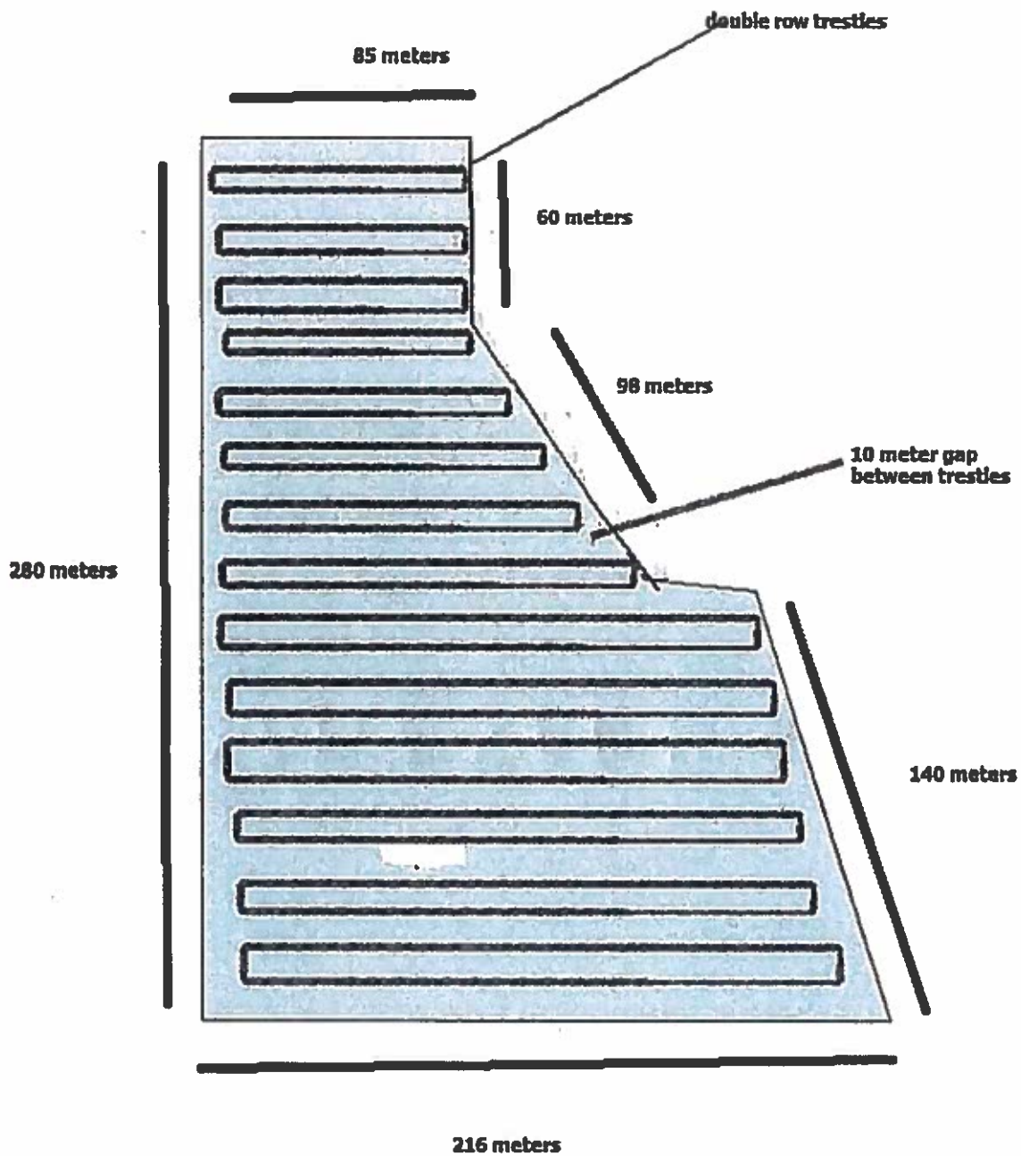
Trestle layout drawing T12/461
